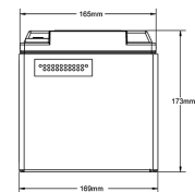
ODS-AGM42LMJ RIGHT POSITIVE FEMALE TERMINALS Metal Jacket
